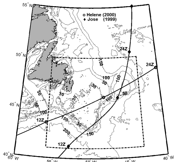
Fig. 2: Map of study area. Newfoundland and Labrador are in grey. Six-hourly storm positions for Tropical Storms Helene and Jose are marked by circles and diamonds, respectively. The contours are shallow water gravity wave speed in m/s. The boundary of the model domain is shown by the dashed box.
